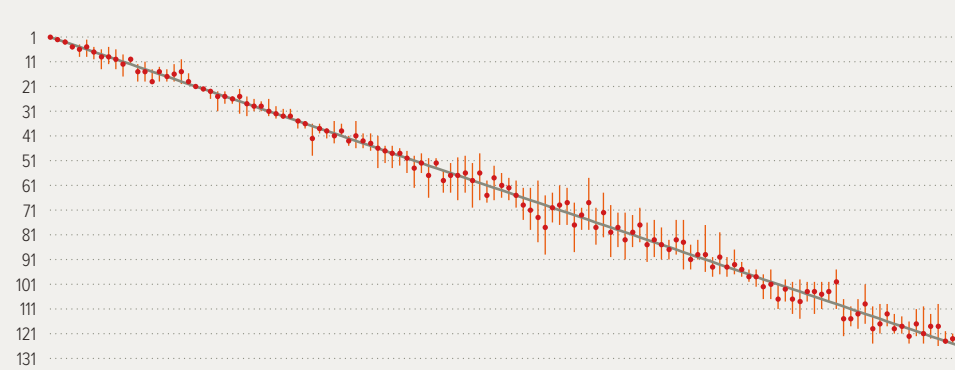
Input rank vs. median rank, 90% confidence intervals
