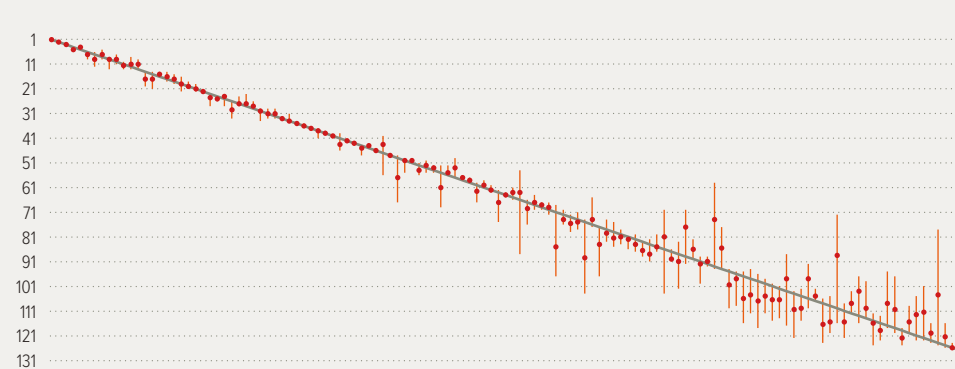
Output rank vs. median rank, 90% confidence intervals
